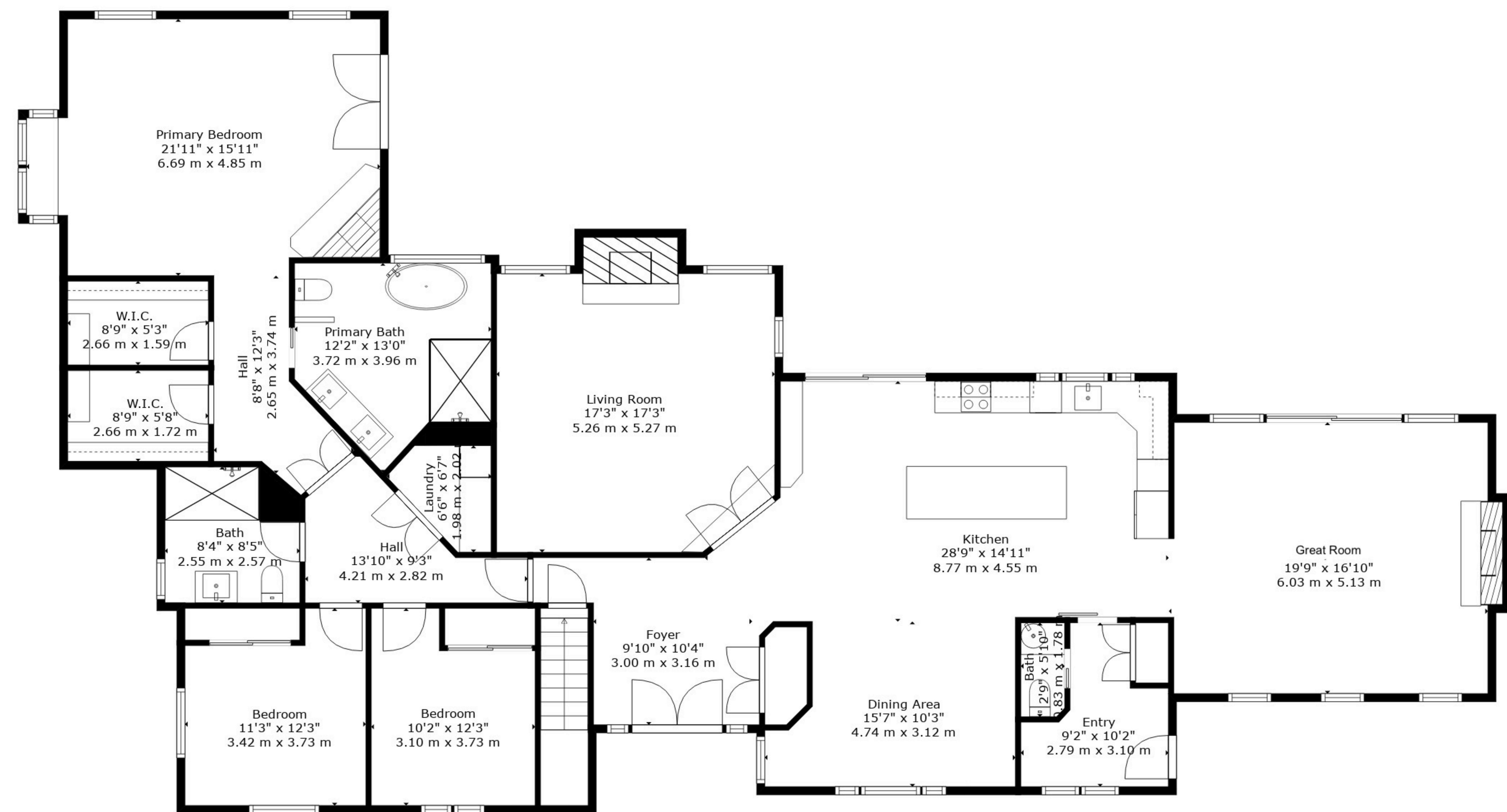
Floor 2
